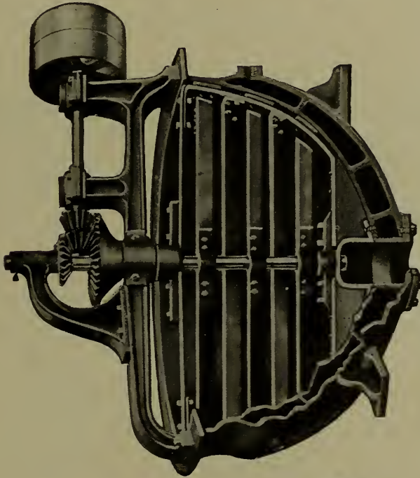
SEAMLESS JACKETED KETTLE equipped with STYLE "D" SAND SOAP MIXER
